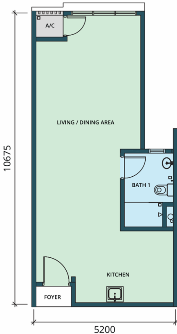
BARE UNIT
