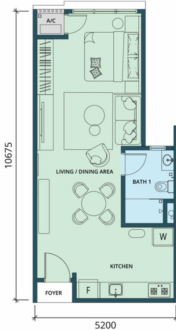
TYPICAL UNIT
